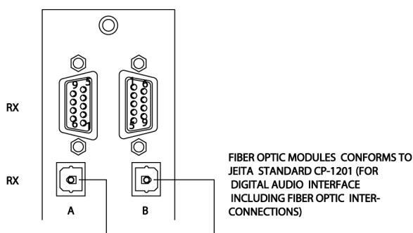
INPUT DIGITAL/DIGITAL MODULE CONNECTIONS
