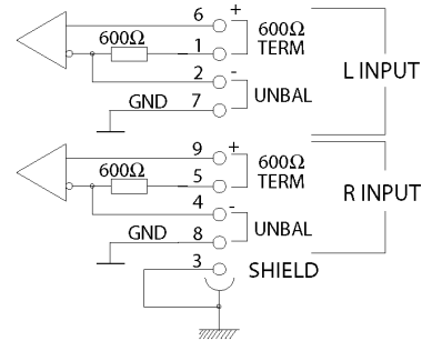
EXT 1 IN
