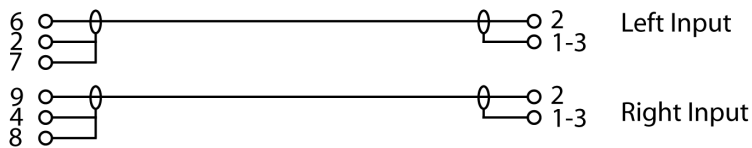
Unbalanced XLR
