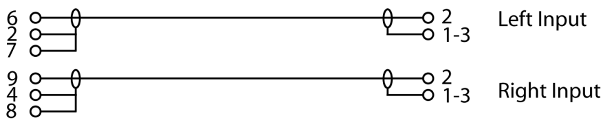
Unbalanced XLR
