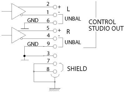
MUTAB.CNTRL STUDIO
