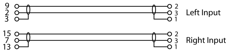
Balanced XLR
